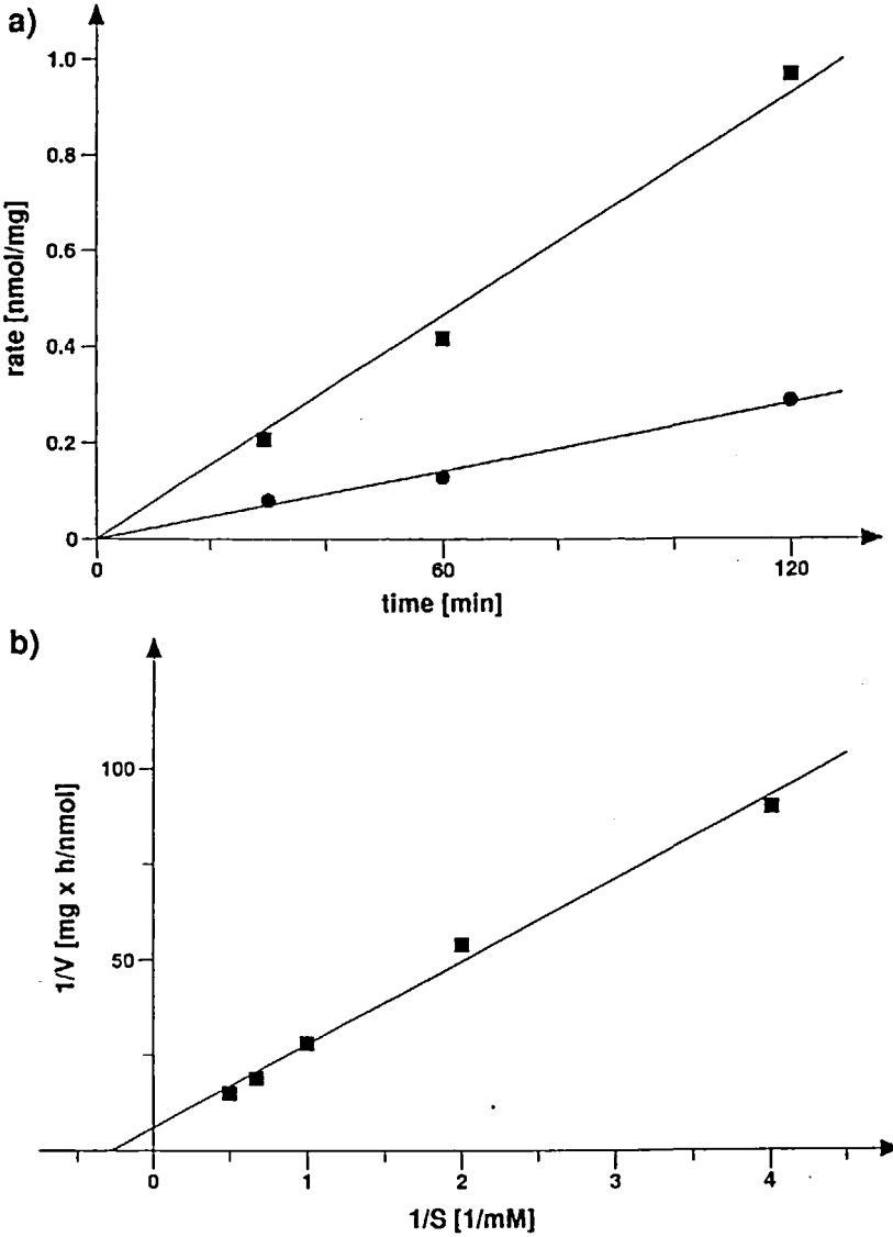
Figure 1. Time dependency (a) and Lineweaver-Burk plot (b) of endomannosidase activity in Golgi preparations from rat liver determined using Glc-Man-Muf as substrate.
